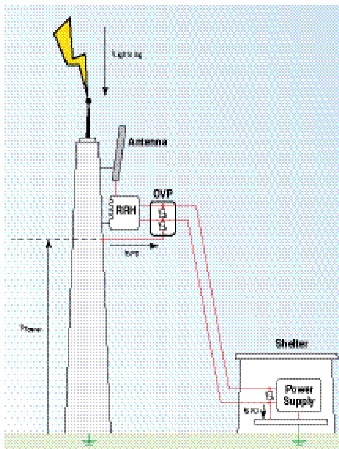
Figure 1. While lightning rods direct the lightning currents down the tower and to the ground, the DC cabling that runs up and down the tower and connects the radios to the power source acts as a direct conduit, bringing the lightning current directly into the equipment. Without the proper surge protective devices installed at critical points, the remote radio head equipment is at high risk of catastrophic failure.
