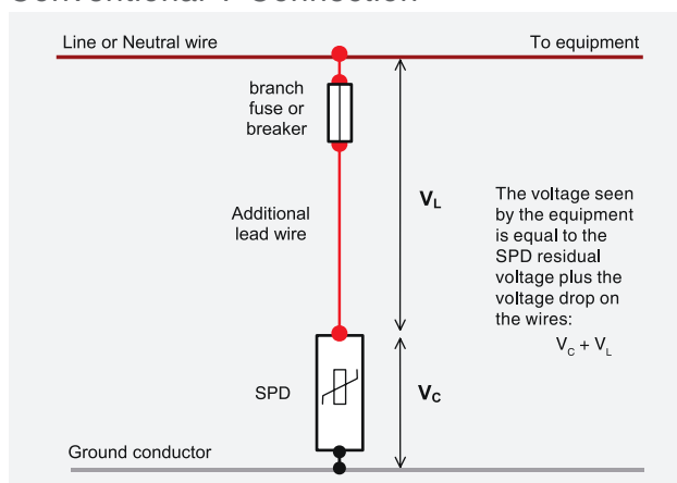
Figure 1: Residual voltage in Kelvin and T-connection applications.
