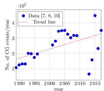
Figure 5: Lightning activity over continental us in past 3 decades.
