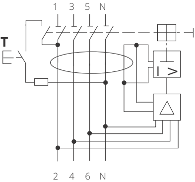
NFI4BK, NFI4BS
