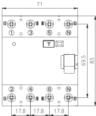
FI4BK FI4BS
