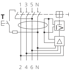
FI4BK, FI4BS
