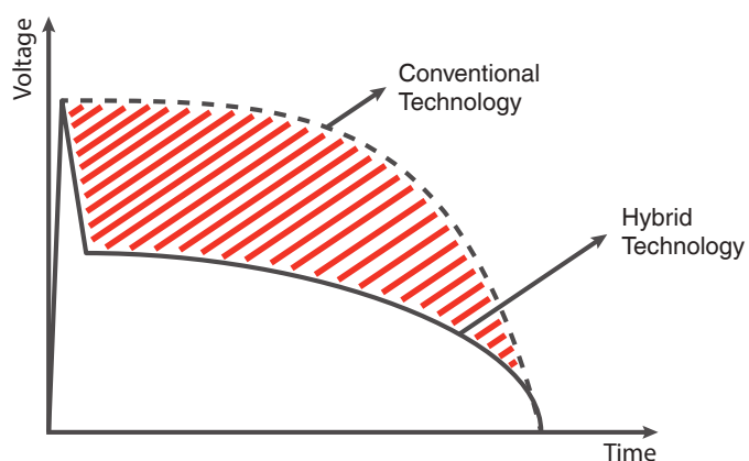
Figure 6: Compared to conventional arrester technology, Raycap's hybrid technology ensures the lowest overvoltage stress on the equipment to be protected.
