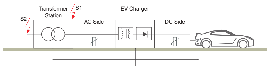
Charging station with various direct lightning strike scenarios (S1/S2) according to IEC 62305.
