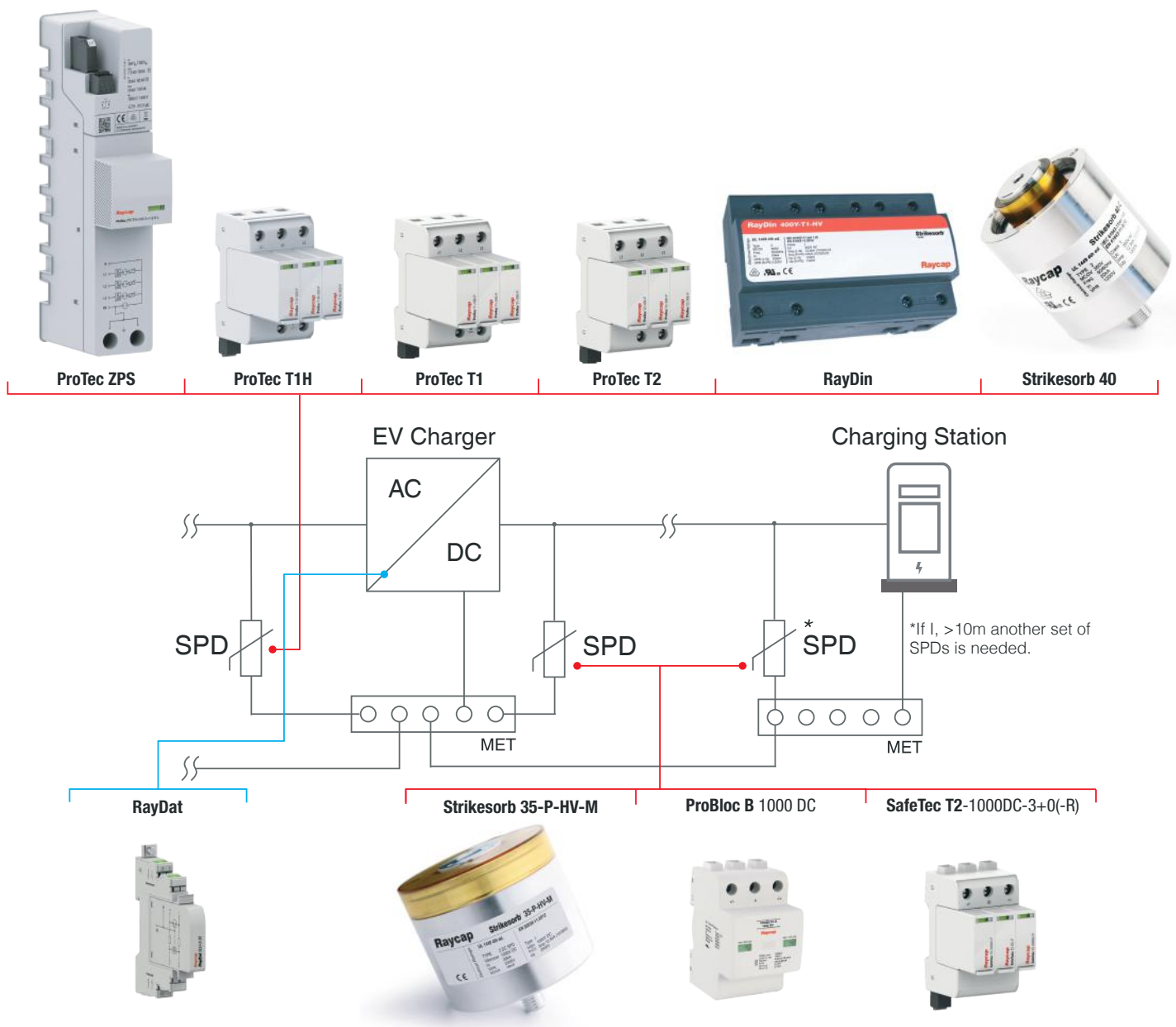
Figure 7: Possible options of lightning and surge protection devices.
