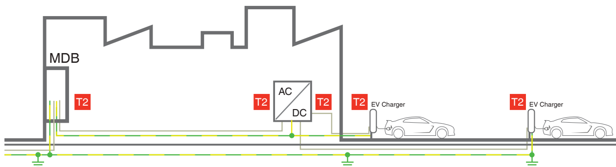
Charging station without LPS with underground power source.
